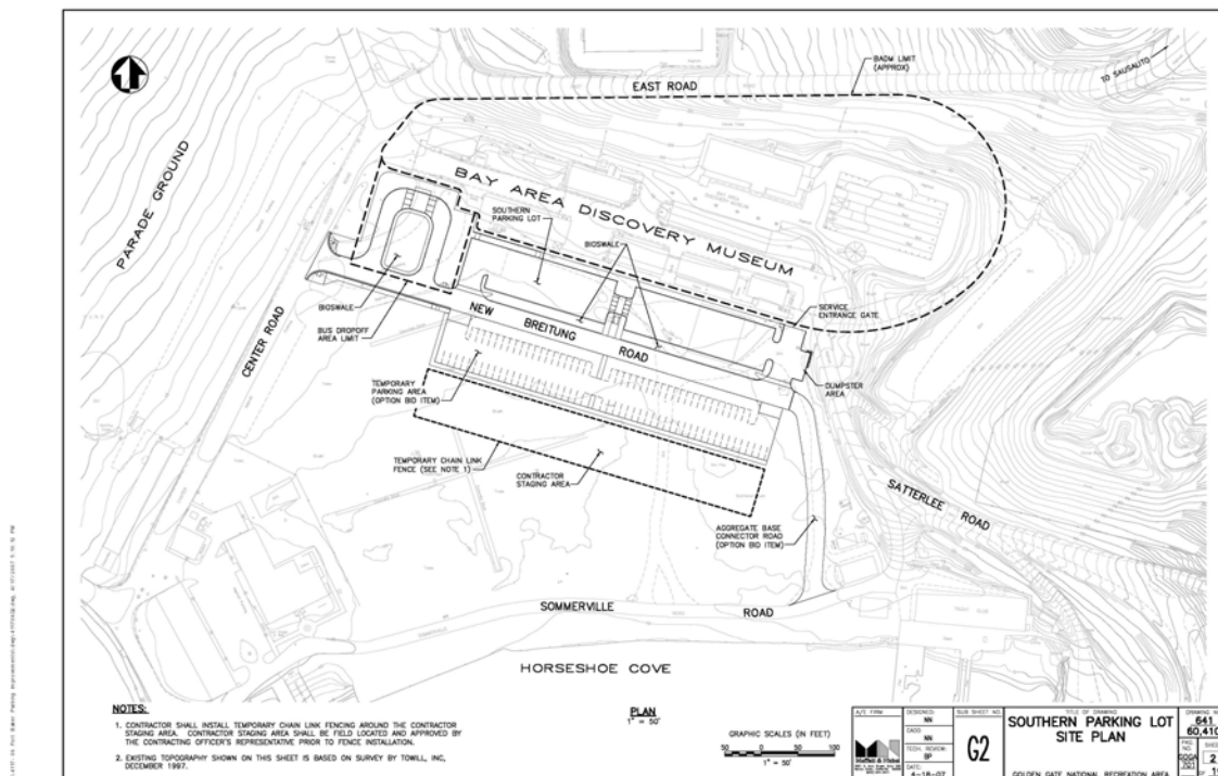
NPS construction plan for the "BADM South Parking Lot" project
